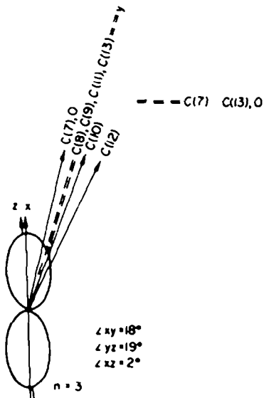
Fig 4. Schematic picture of directions of \pi -orbitals of polyenic chain of I ( n = 3 , R = \text{Br} ).
