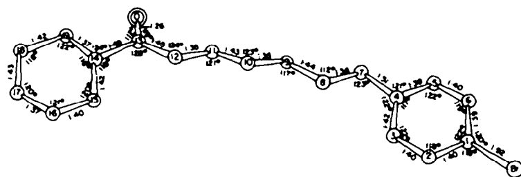
Fig 2. The projection of the molecule of I ( n = 3 , R = \text{Br} ) on the plane (X, Y, 0)
