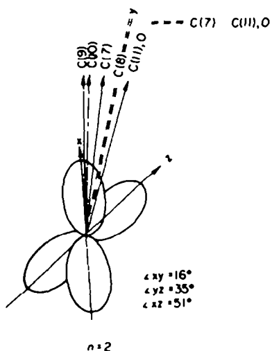
Fig 3. Schematic picture of directions of \pi -orbitals of polyenic chain of I ( n = 2 , R = \text{Br} ).
