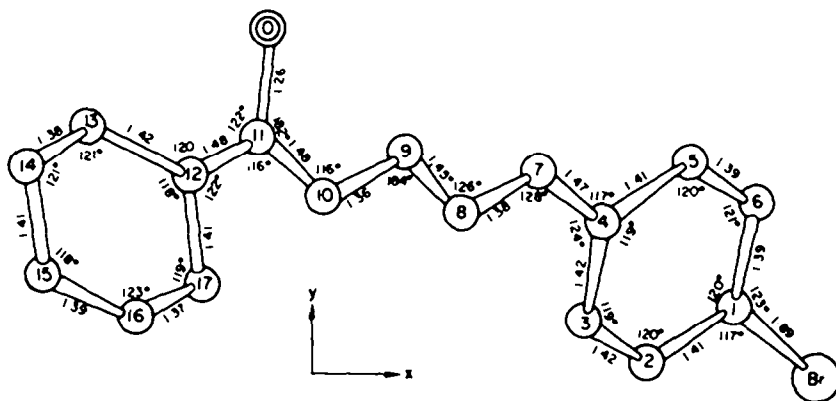
Fig 1. The projection of the molecule of I ( n = 2 , R = \text{Br} ) on the plane (X, Y, 0)
